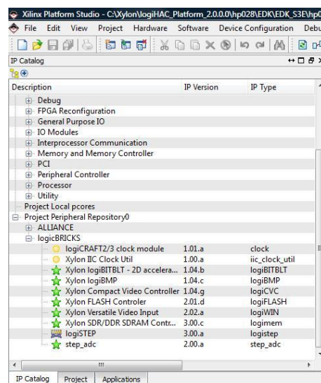
Figure 3: The logicBRICKS in the EDK IP Catalogue
